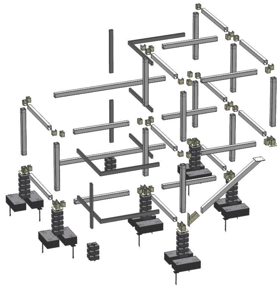
EXPLODED VIEW
