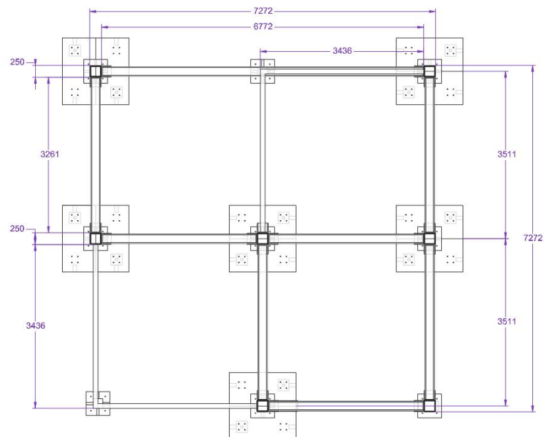
STRUCTURAL PLAN
