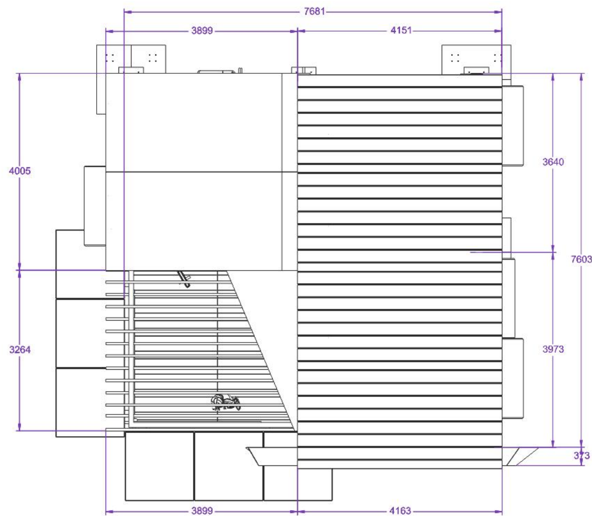
ROOF PLAN
